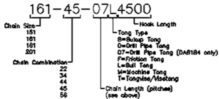
THIS IS WHAT A CHAIN PART NUMBER TELLS YOU
