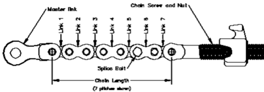
CHAIN ASSEMBLY
